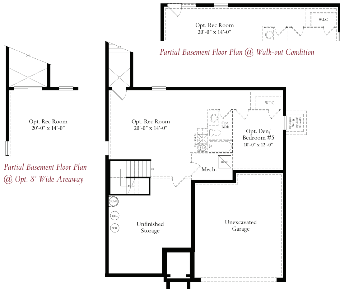
Opt. Partial Basement Floor Plan @ Opt. 4' Great Room Extension Above w/ Opt. 8' Wide Areaway
